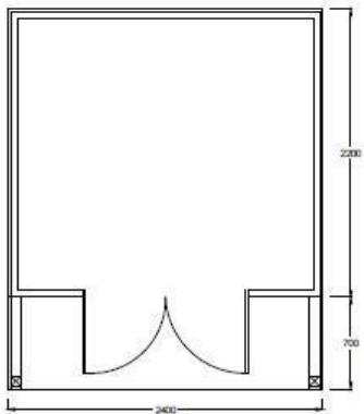
PROPOSED BEACH HUT PLAN
