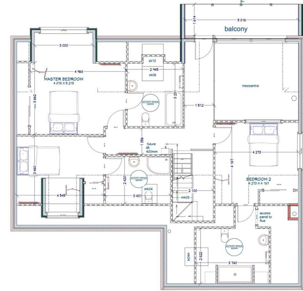
first floor plan view
