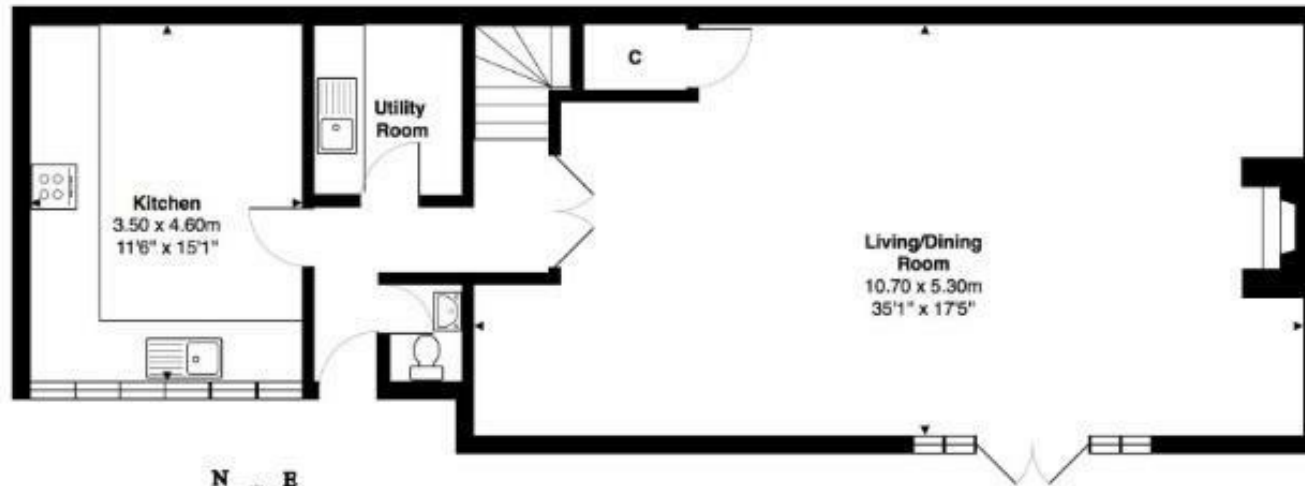
Ground Floor
