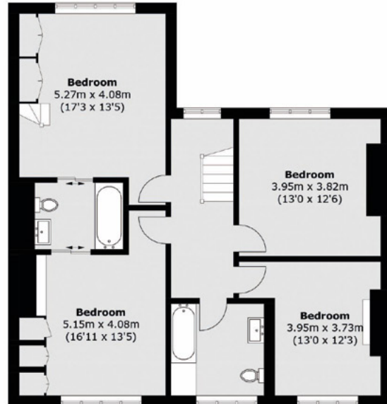
Second Floor
