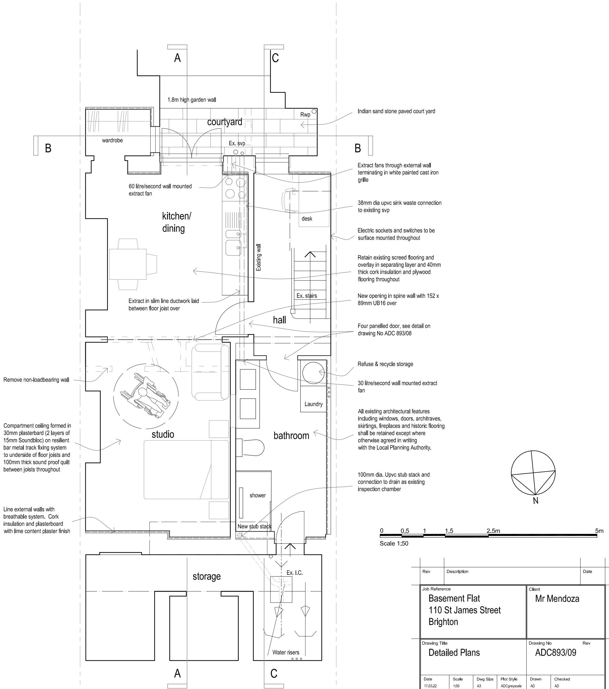
Basement Plan @ 1:50
