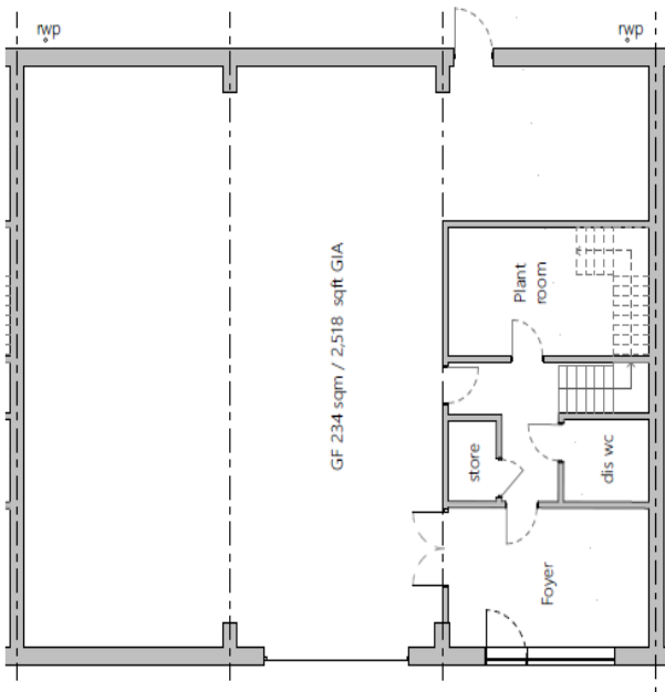
UNITS 13 - 14 TYPICAL GROUND FLOOR PLAN
