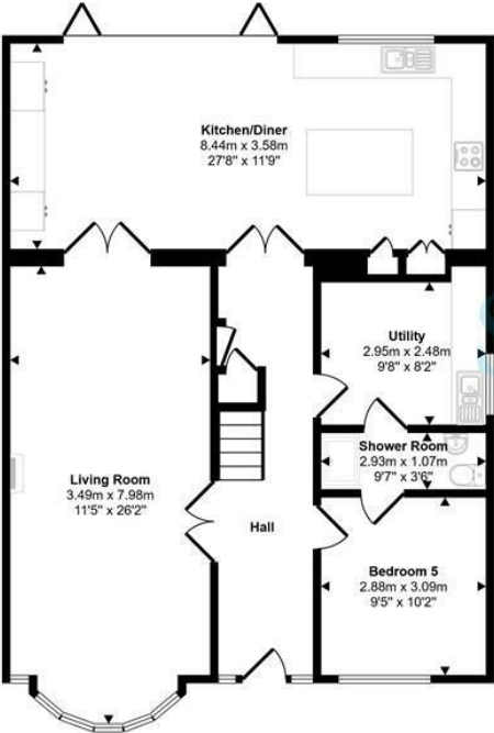
Ground Floor Approx 94 sq m / 1017 sq ft
