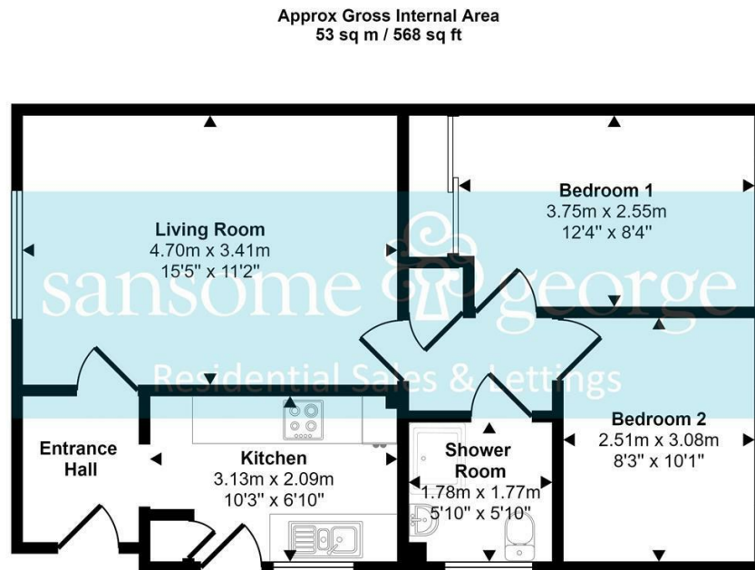
Floorplan
