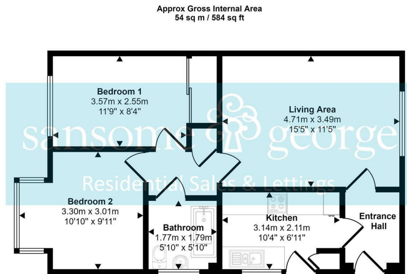
Floorplan
