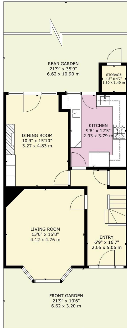
GROUND FLOOR
