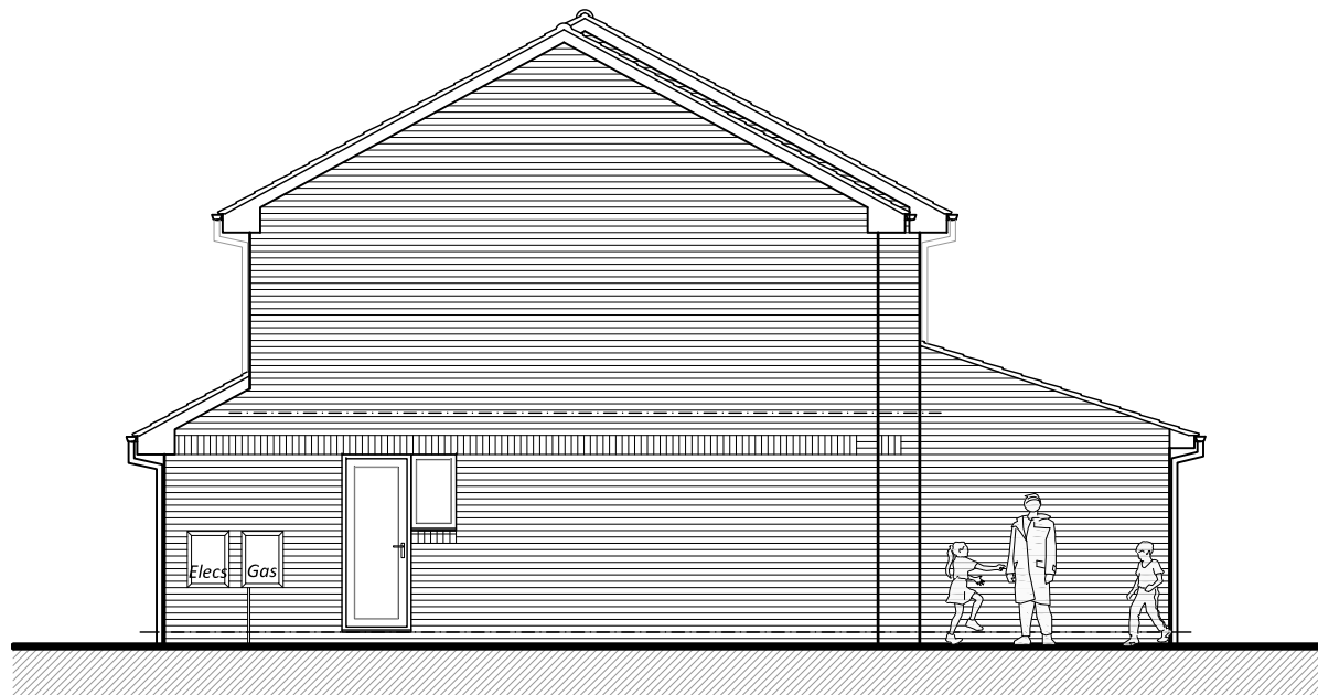
02 NORTH WEST ELEVATION 1:100
