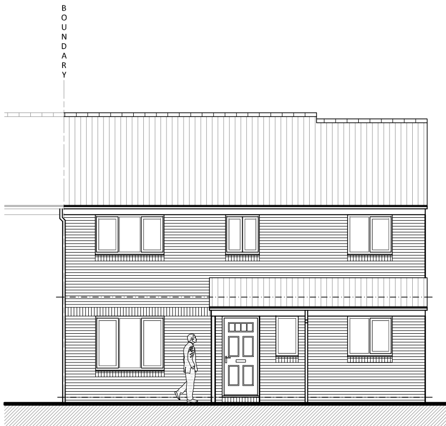
01 NORTH EAST ELEVATION 1:100
