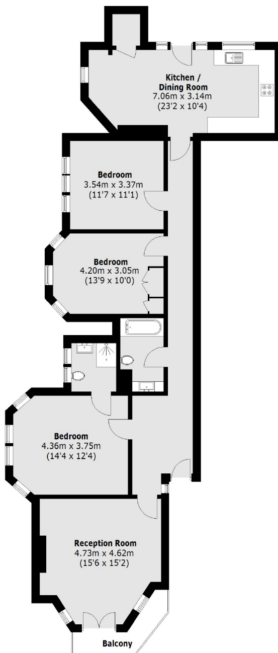
Second Floor
