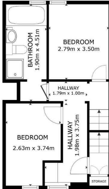
FLOOR 2
