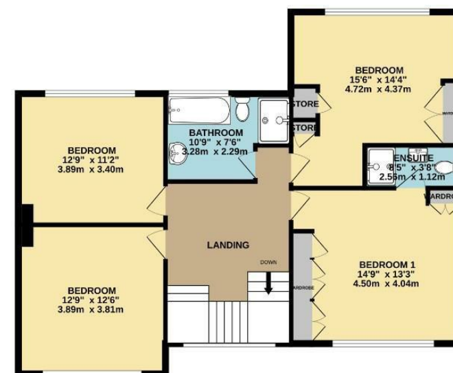
1ST FLOOR 946 sq.ft. (87.9 sq.m.) approx.
