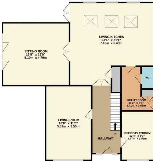
GROUND FLOOR 1196 sq.ft. (111.0 sq.m.) approx.
