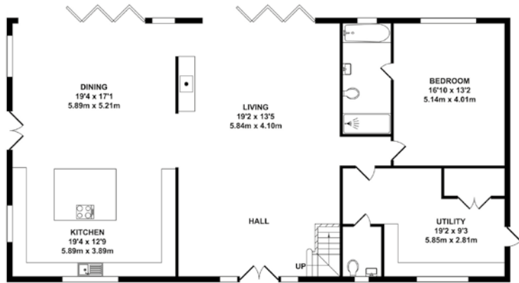
GROUND FLOOR 1751 sq.ft / 162.69 sq.m
