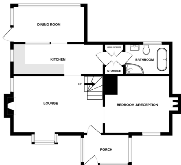
GROUND FLOOR 601 sq.ft. (55.8 sq.m.) approx.
