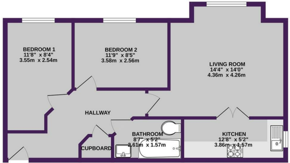
GROUND FLOOR 609 sq.ft. (56.5 sq.m.) approx.
