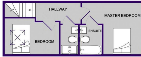
1ST FLOOR
