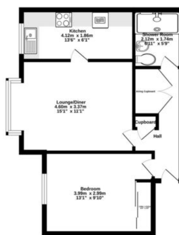
2nd Floor 44.6 sq.m. (480 sq.ft.) approx.
