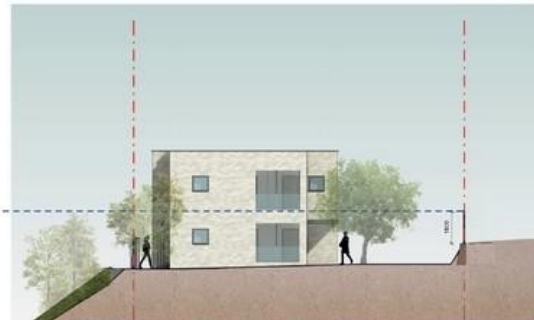
Block A South Elevation 1:100
