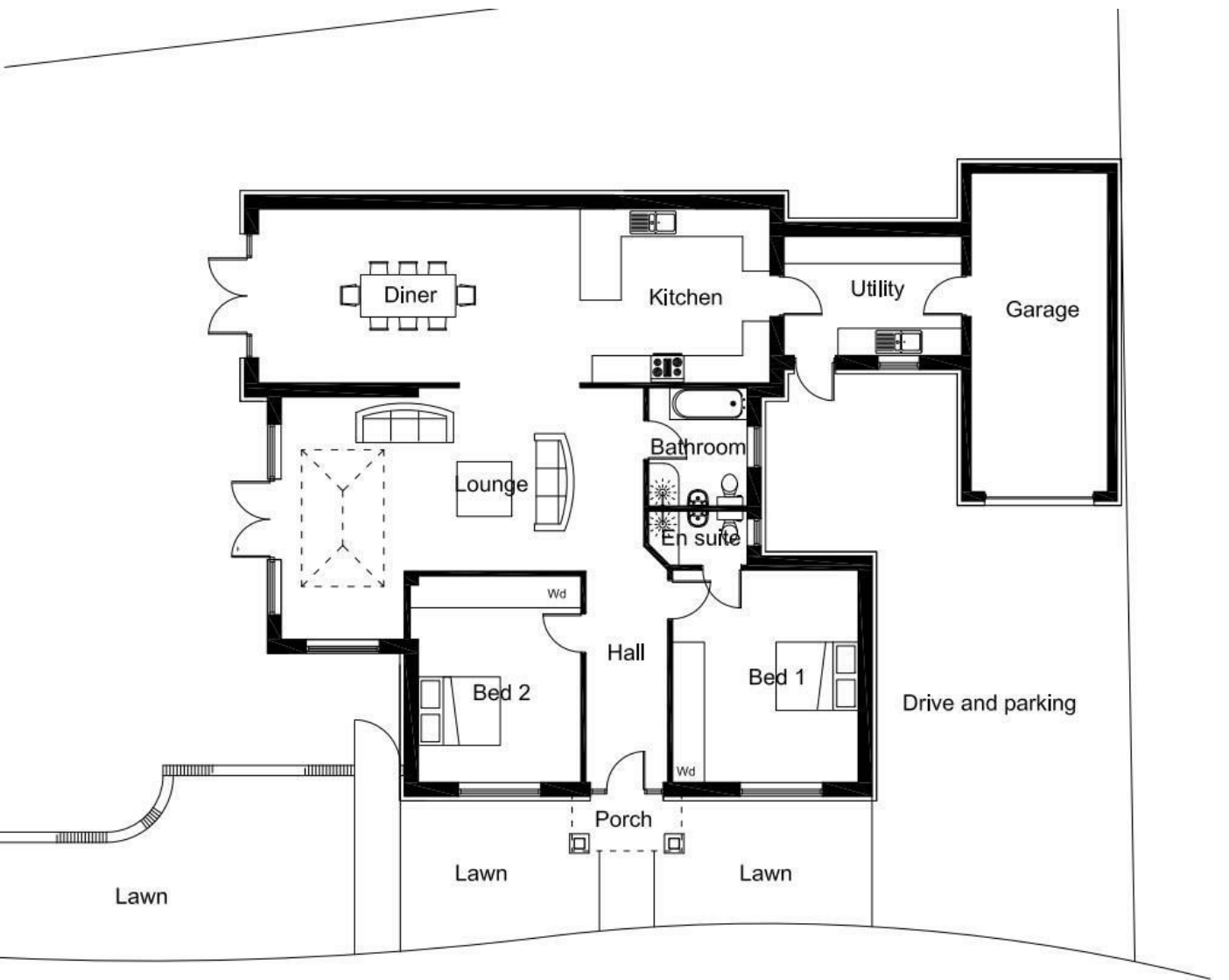
Proposed Bungalow 163 m2 - 1754 ft2
