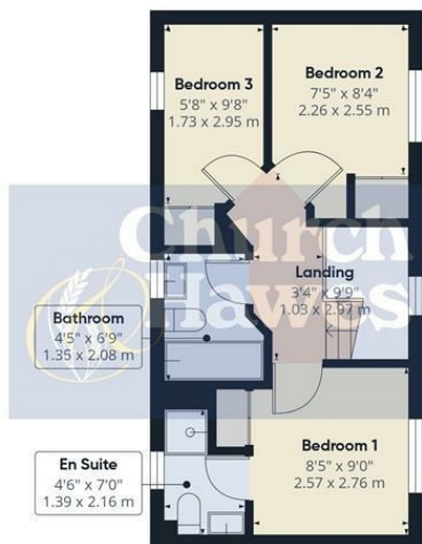
Floor 1 Building 1
