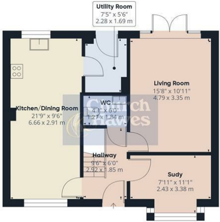
Floor 0 Building 1
