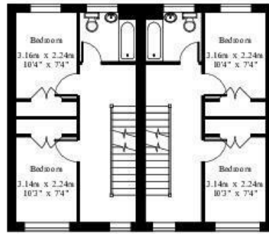
Plot 1 First Floor Plot 2
