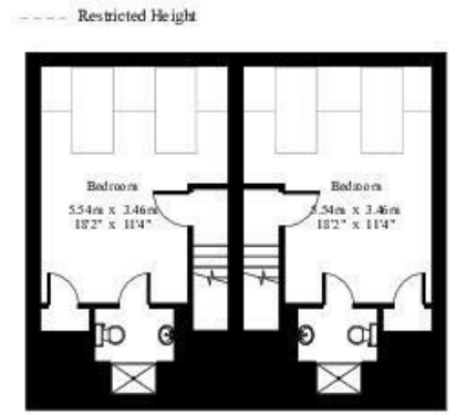
Plot 1 Second Floor Plot 2
