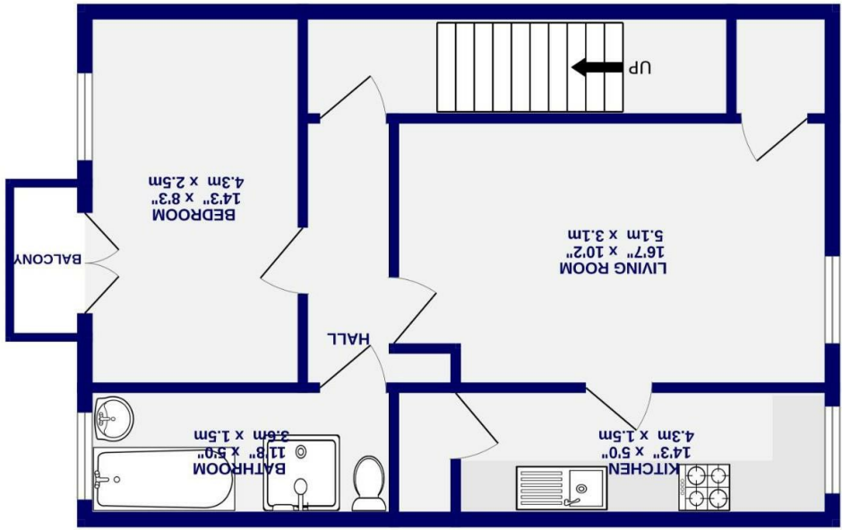
1ST FLOOR 542 sq.ft. (50.4 sq.m.) approx.
