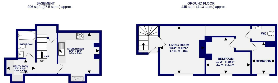
TOTAL FLOOR AREA : 740 sq.ft. (68.8 sq.m.) approx.
