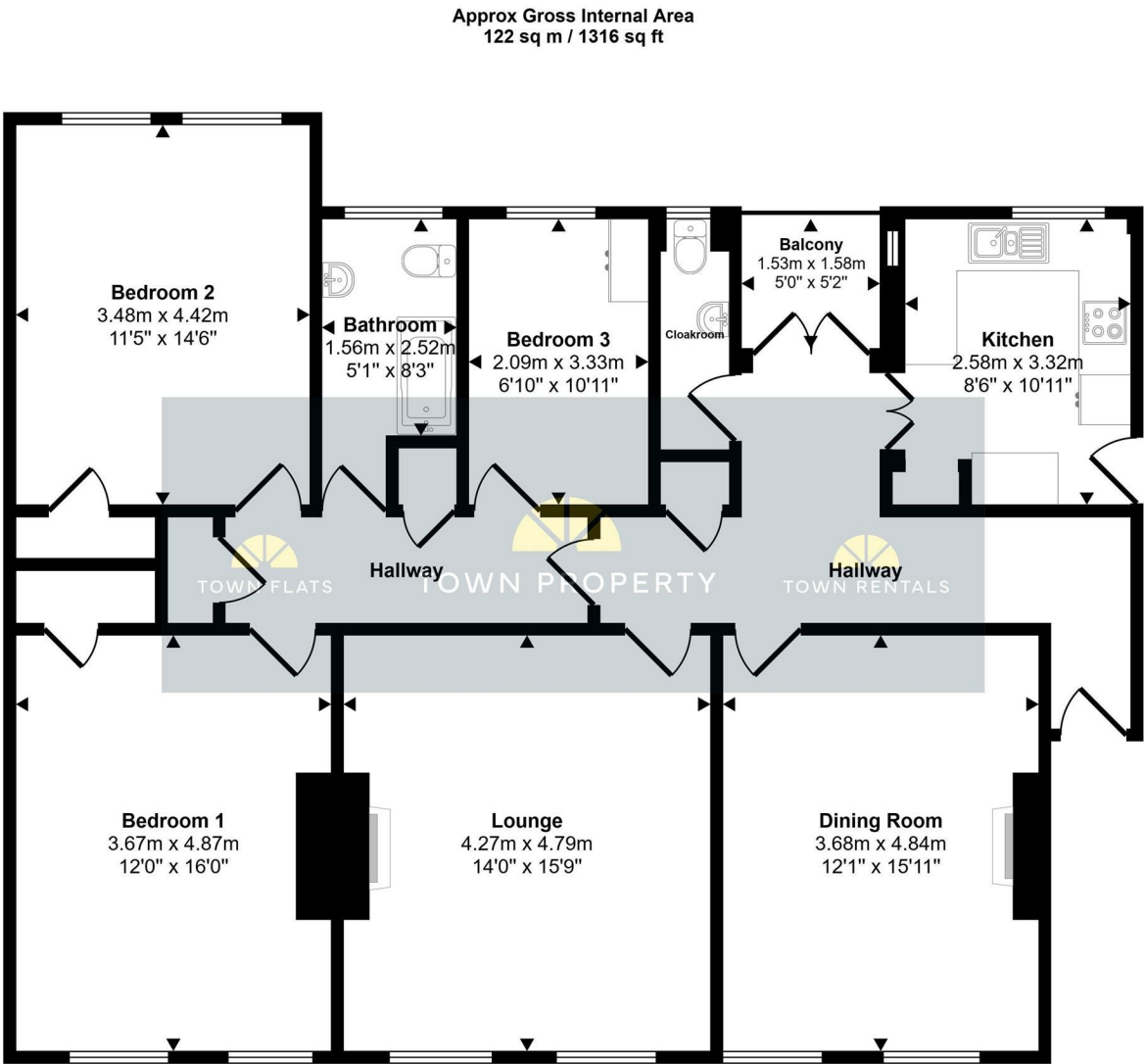
Floorplan
