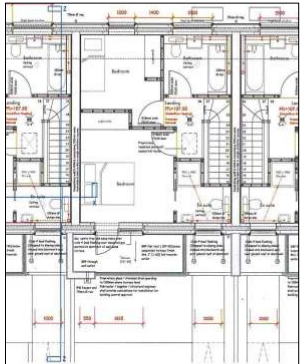
SECOND FLOOR
