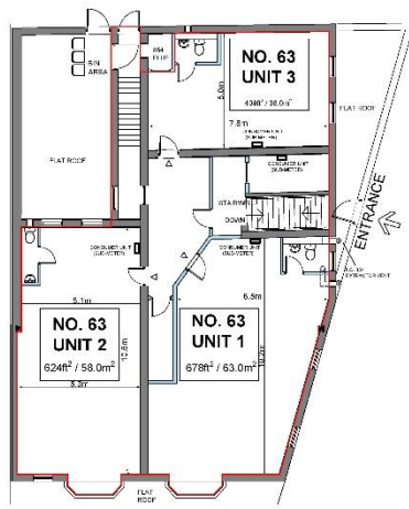
FIRST FLOOR - 63 THORNTON RD
