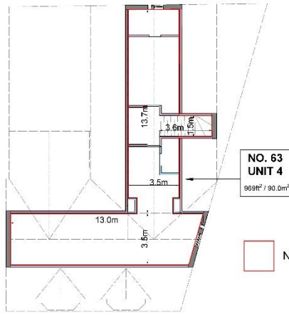
SECOND FLOOR - 63 THORNTON RD
