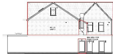
REAR ELEVATION
