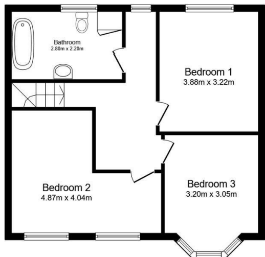
First Floor Floor area 58.5 sq.m.
