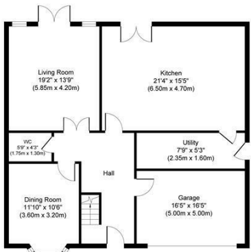
Ground Floor Approximate Floor Area 1145 sq. ft (106.41 sq. m)
