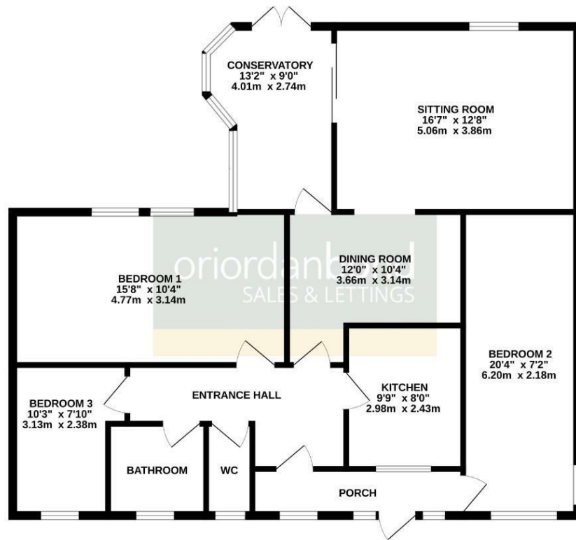
GROUND FLOOR 1104 sq.ft. (102.5 sq.m.) approx.
