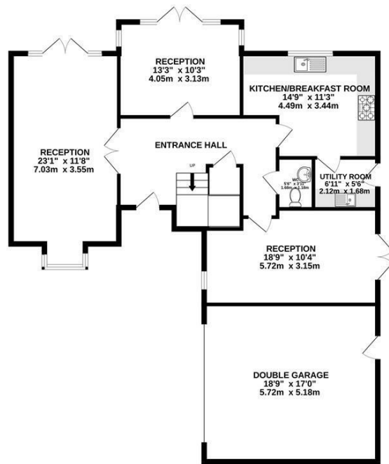
GROUND FLOOR 1285 sq.ft. (119.4 sq.m.) approx.
