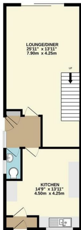
GROUND FLOOR 566 sq ft (52.0 sq m) approx.
