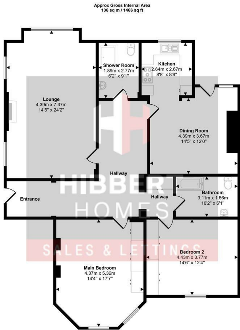
Floorplan
