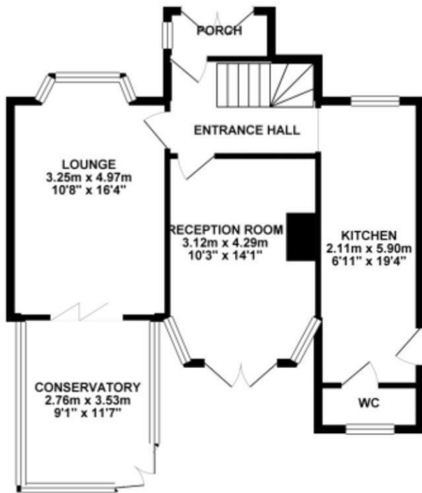
GROUND FLOOR 60.57 sq. m. ( 652.02 sq. ft. )
