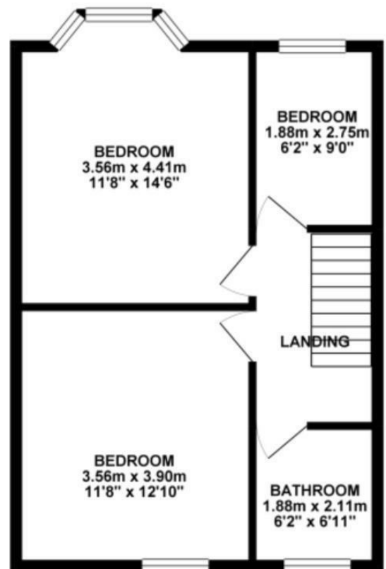
1ST FLOOR 43.37 sq. m. ( 466.81 sq. ft. )
