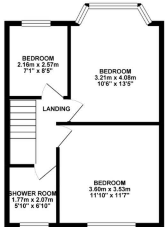
1ST FLOOR 38.90 sq. m. ( 418.73 sq. ft. )
