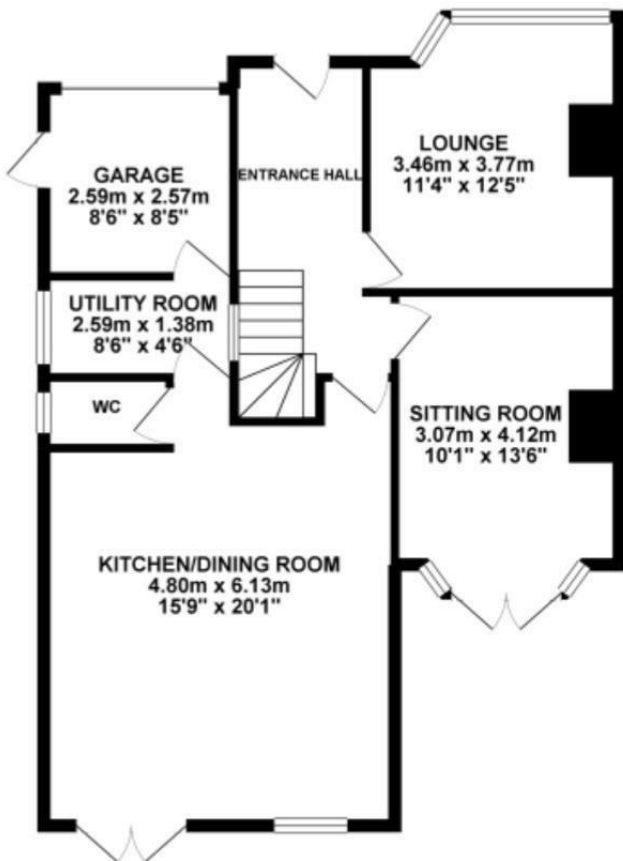
GROUND FLOOR 72.63 sq. m. ( 781.81 sq. ft. )
