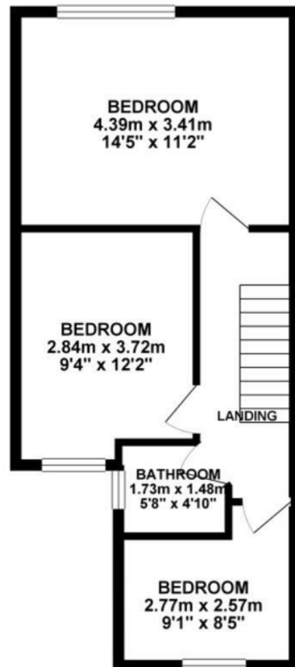
1ST FLOOR 40.02 sq. m. ( 430.78 sq. ft. )
