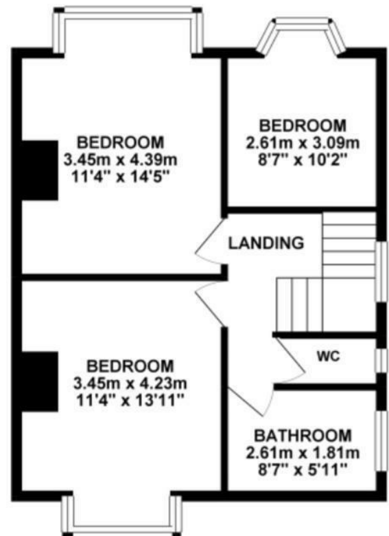
1ST FLOOR 50 sq. m. ( 538.20 sq. ft. )
