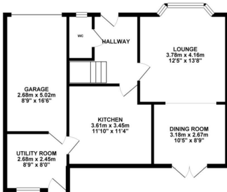
GROUND FLOOR 64.58 sq. m. ( 695.09 sq. ft. )
