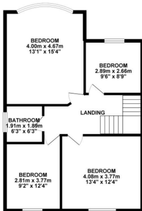
1ST FLOOR 64.91 sq. m. ( 698.66 sq. ft. )
