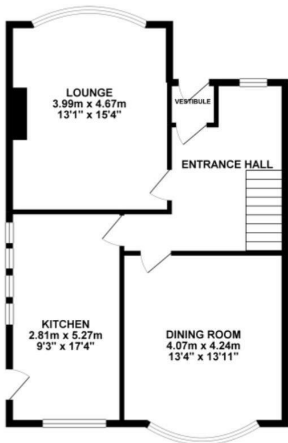
GROUND FLOOR 65.75 sq. m. ( 707.76 sq. ft. )
