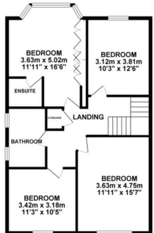
1ST FLOOR 75.76 sq. m. ( 815.52 sq. ft. )
