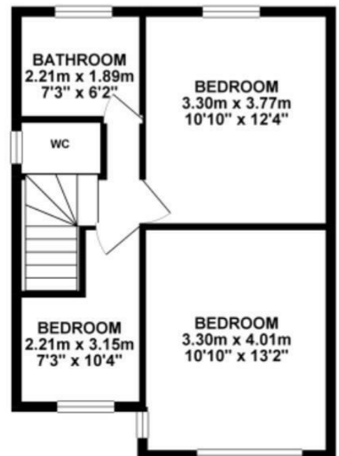
1ST FLOOR 40.99 sq. m. ( 441.23 sq. ft. )
