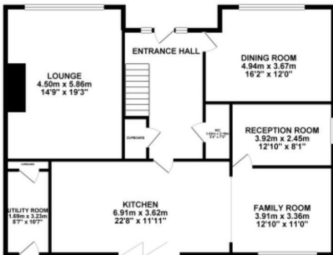
GROUND FLOOR 115.40 sq. m. ( 1242.19 sq. ft. )
