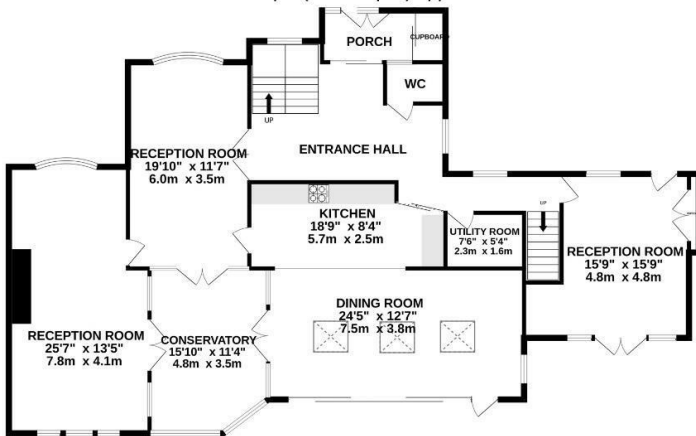
GROUND FLOOR 1795 sq.ft. (166.8 sq.m.) approx.
