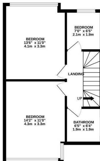
1ST FLOOR 450 sq.ft. (41.8 sq.m.) approx.
