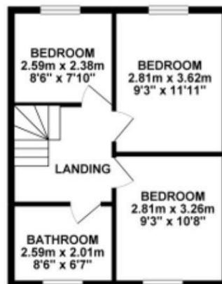
1ST FLOOR 37.21 sq. m. ( 400.52 sq. ft. )
